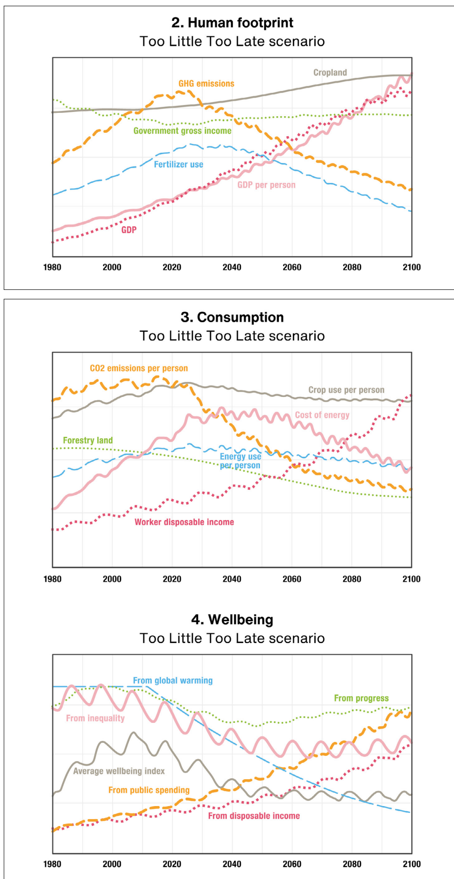
Figure 6: Key trends describing the Too Little Too Late scenario.
